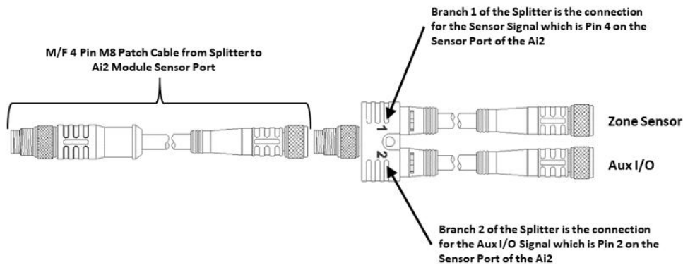
Typical Parallel Splitter Cable Usage
